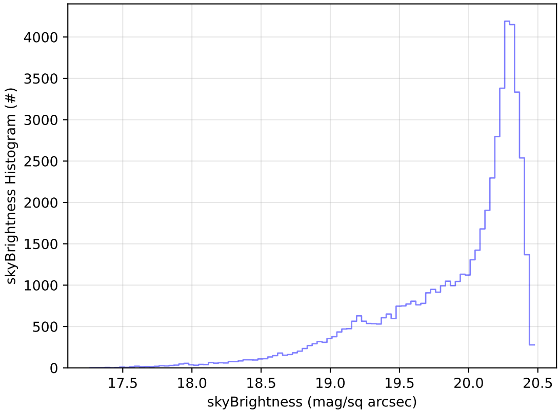
start_date_do-270v3.4_10yrs Yr 1 i band: skyBrightness Histogram
