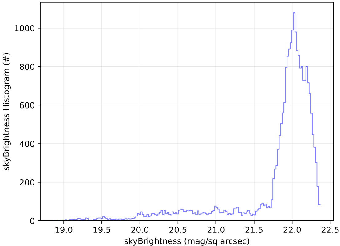
start_date_do-270v3.4_10yrs Yr 1 g band: skyBrightness Histogram
