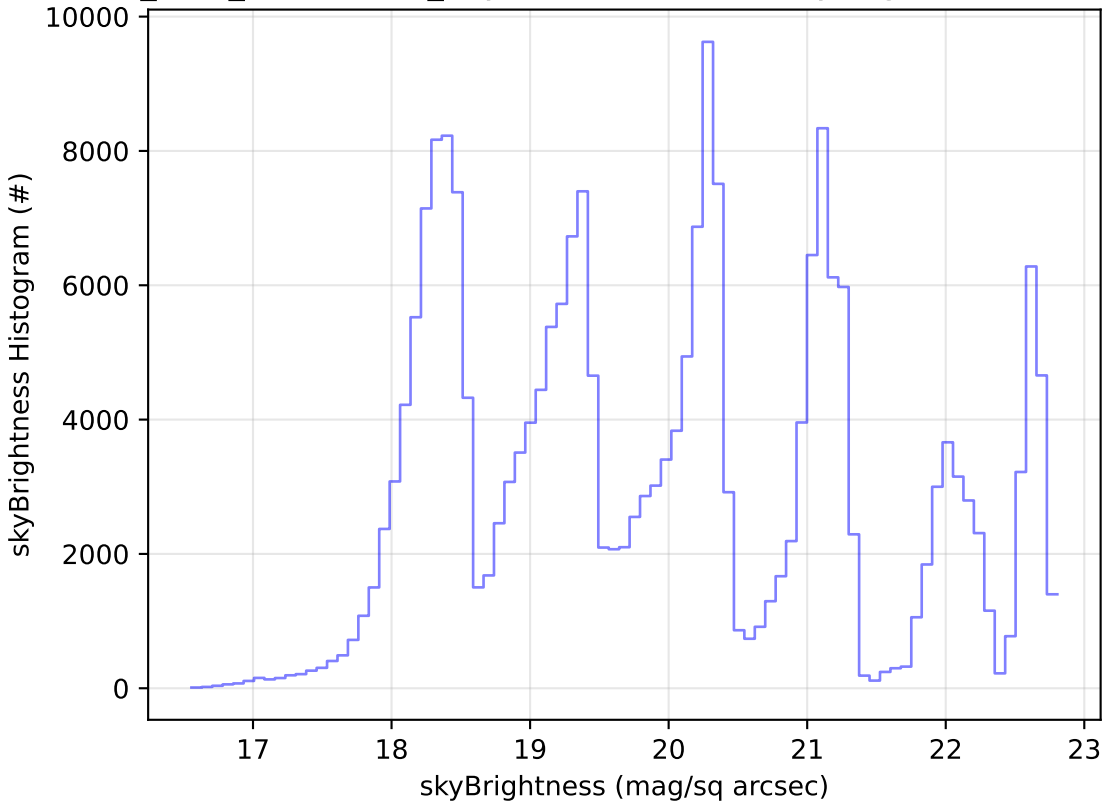
start_date_do-270v3.4_10yrs Yr 1 all bands: skyBrightness Histogram
