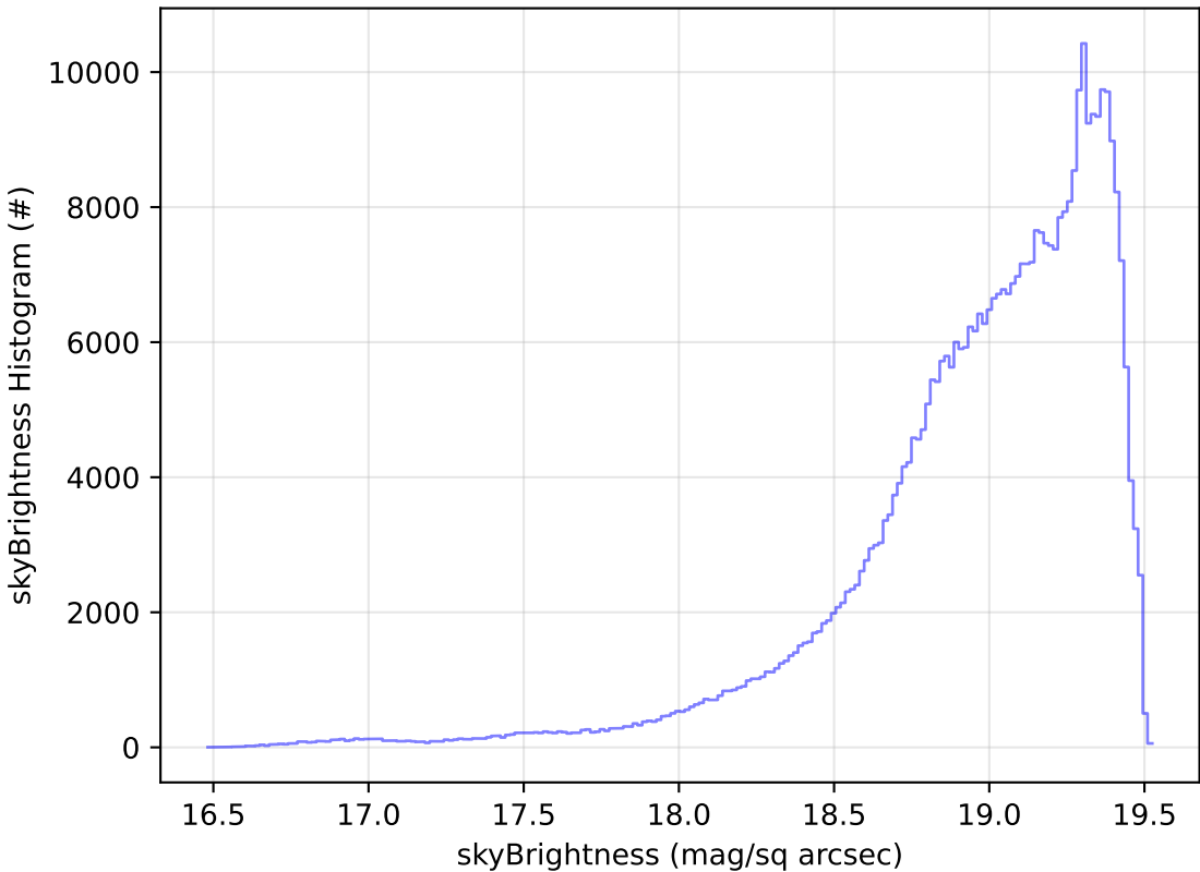
start_date_do-270v3.4_10yrs WFD z band: skyBrightness Histogram
