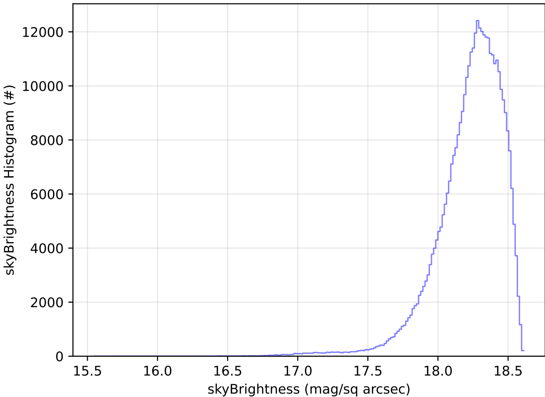
start_date_do-270v3.4_10yrs WFD y band: skyBrightness Histogram
