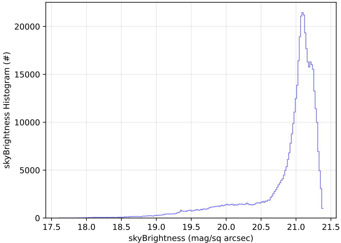
start_date_do-270v3.4_10yrs WFD r band: skyBrightness Histogram
