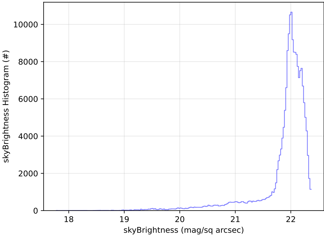
start_date_do-270v3.4_10yrs WFD g band: skyBrightness Histogram
