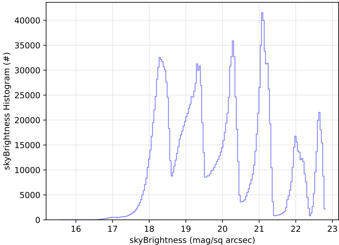
start_date_do-270v3.4_10yrs WFD all bands: skyBrightness Histogram
