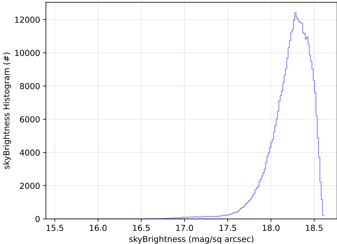
start_date_do-270v3.4_10yrs All sky y band: skyBrightness Histogram
