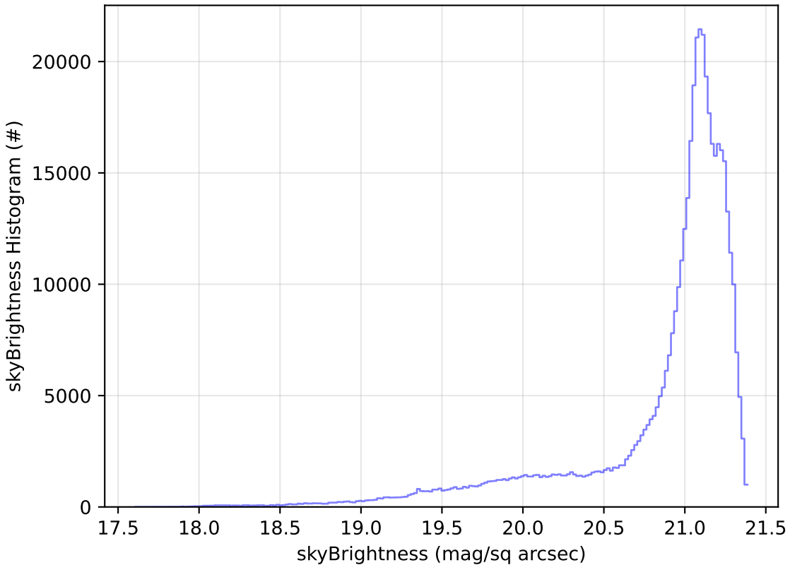
start_date_do-270v3.4_10yrs All sky r band: skyBrightness Histogram
