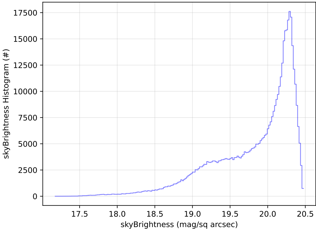
start_date_do-270v3.4_10yrs All sky i band: skyBrightness Histogram
