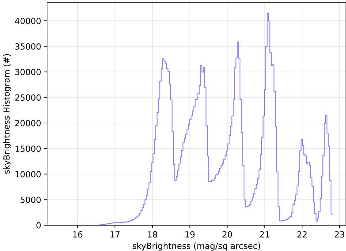
start_date_do-270v3.4_10yrs All sky all bands: skyBrightness Histogram
