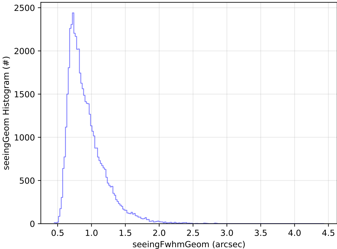
start_date_do-270v3.4_10yrs Yr 1 r band: seeingGeom Histogram
