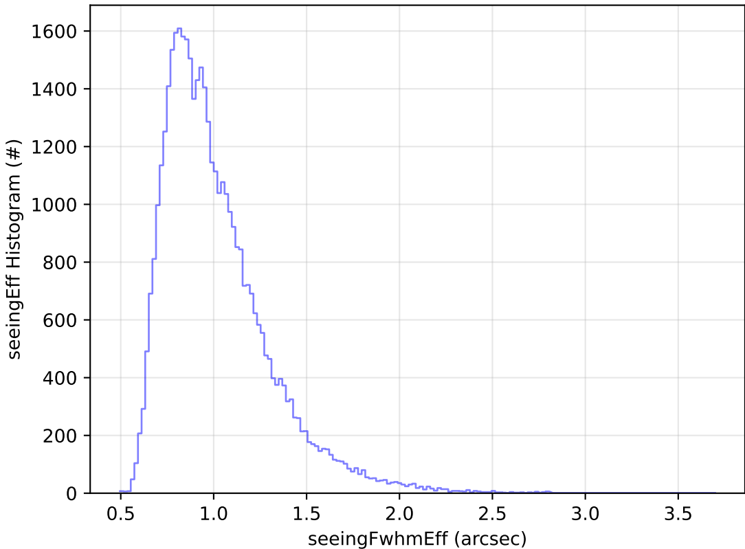
start_date_do-270v3.4_10yrs Yr 1 z band: seeingEff Histogram
