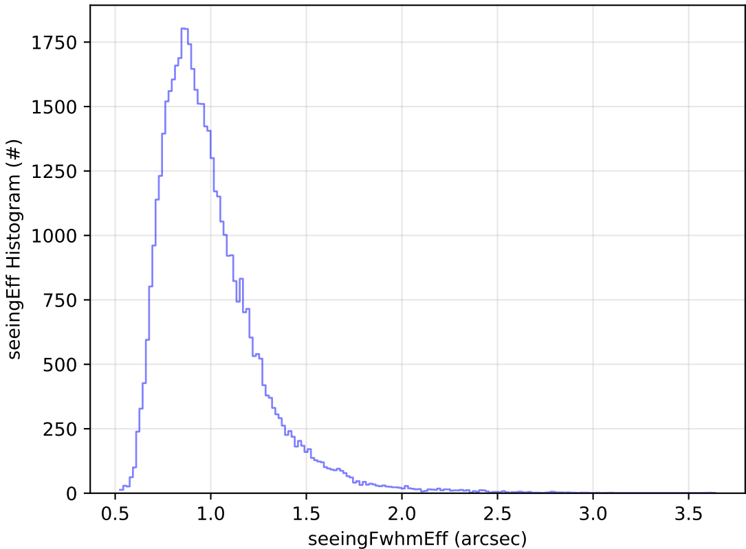
start_date_do-270v3.4_10yrs Yr 1 y band: seeingEff Histogram
