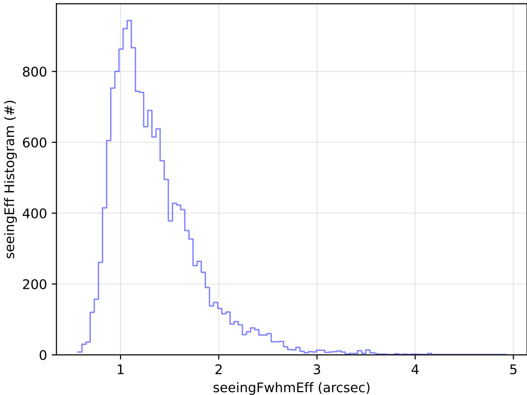
start_date_do-270v3.4_10yrs Yr 1 u band: seeingEff Histogram
