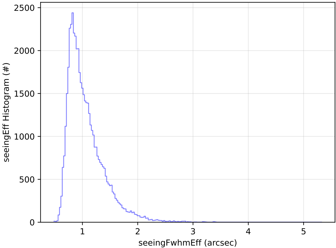
start_date_do-270v3.4_10yrs Yr 1 r band: seeingEff Histogram
