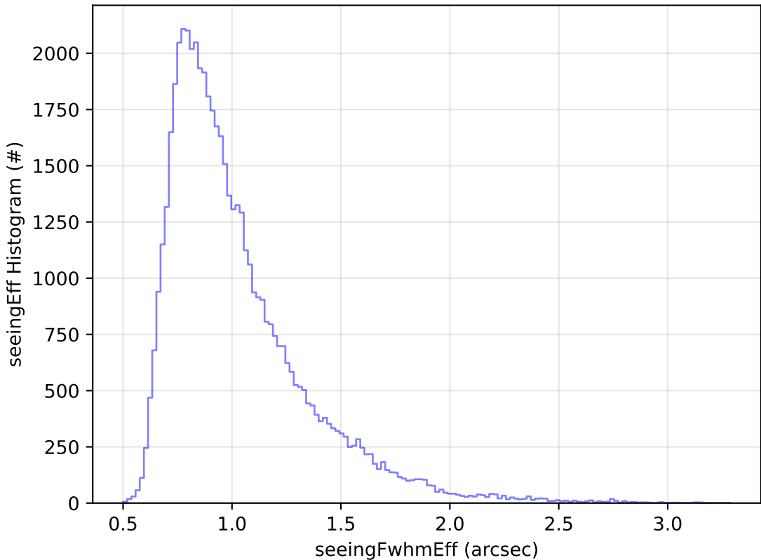
start_date_do-270v3.4_10yrs Yr 1 i band: seeingEff Histogram
