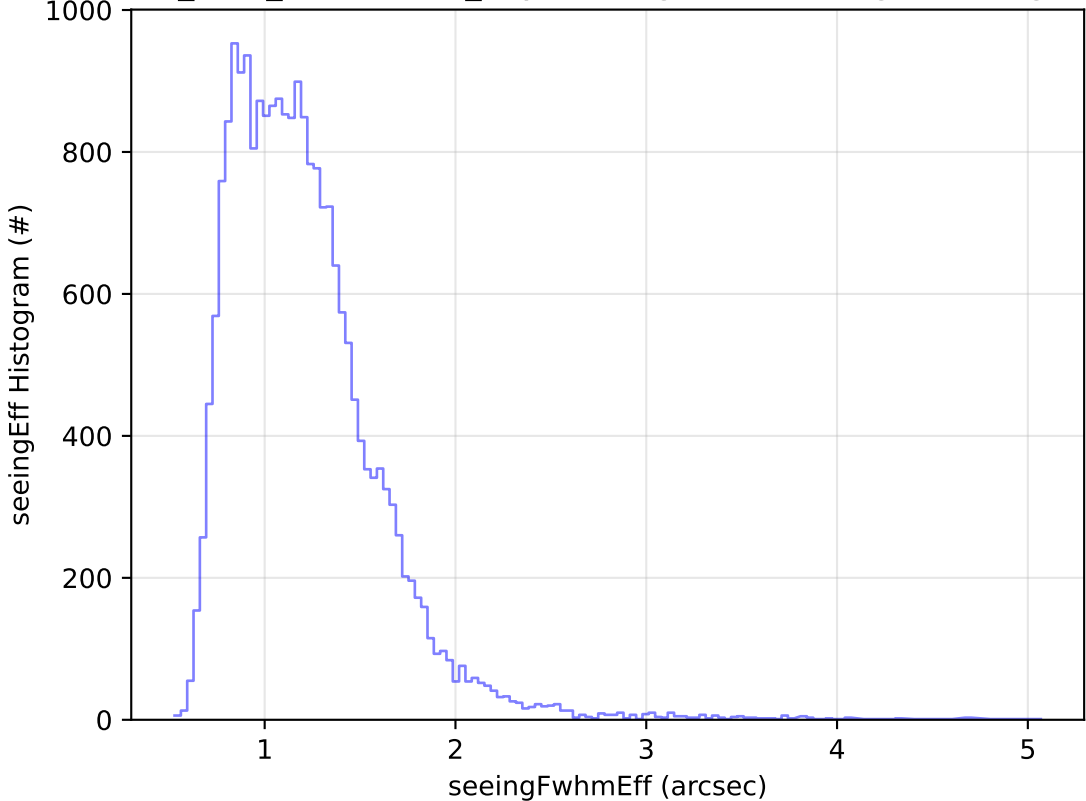
start_date_do-270v3.4_10yrs Yr 1 g band: seeingEff Histogram
