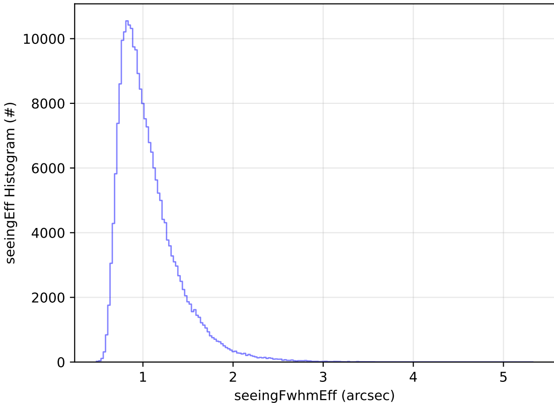
start_date_do-270v3.4_10yrs Yr 1 all bands: seeingEff Histogram
