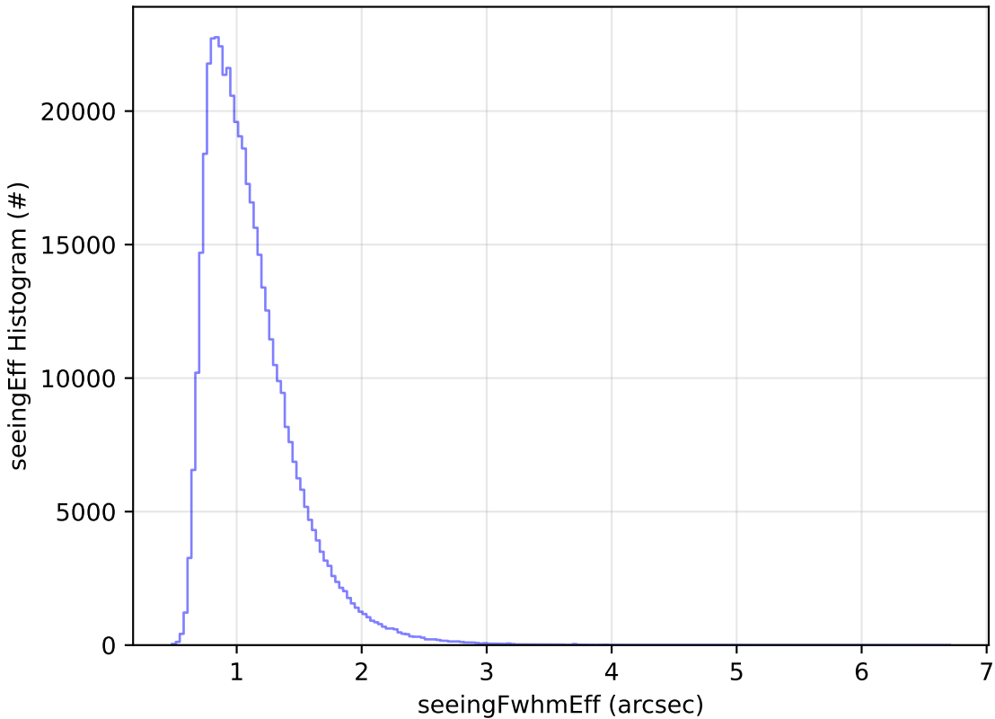
start_date_do-270v3.4_10yrs WFD r band: seeingEff Histogram
