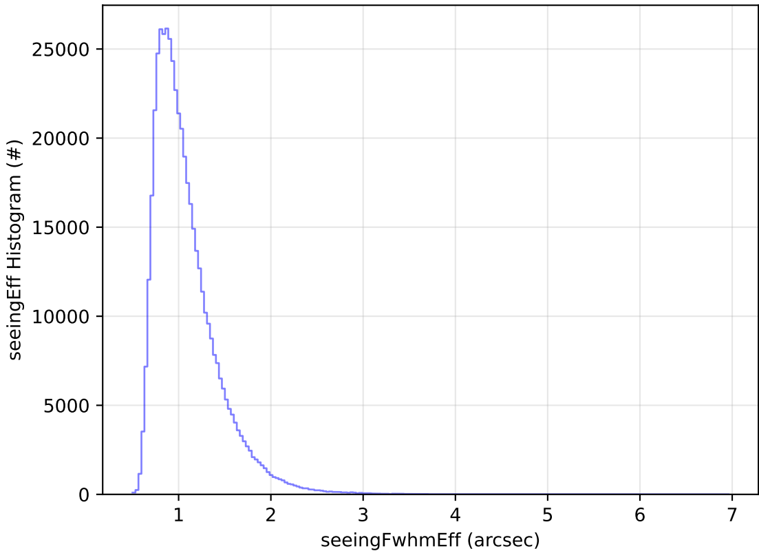
start_date_do-270v3.4_10yrs WFD i band: seeingEff Histogram
