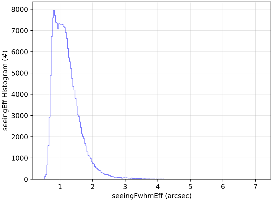
start_date_do-270v3.4_10yrs WFD g band: seeingEff Histogram
