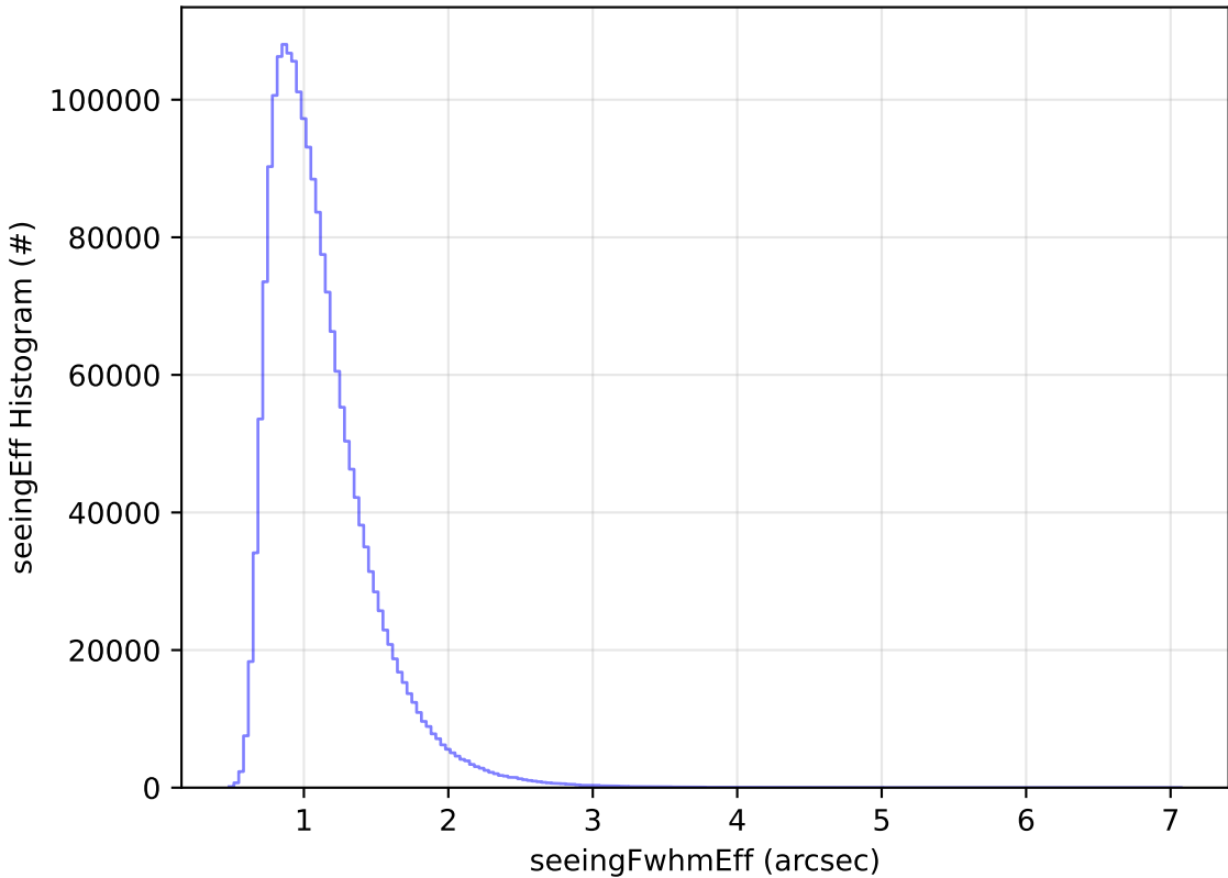
start_date_do-270v3.4_10yrs WFD all bands: seeingEff Histogram
