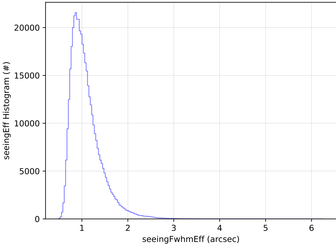
start_date_do-270v3.4_10yrs All sky z band: seeingEff Histogram
