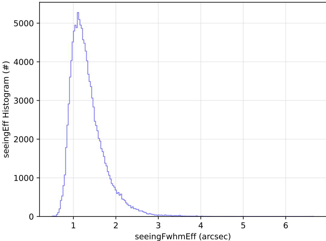
start_date_do-270v3.4_10yrs All sky u band: seeingEff Histogram
