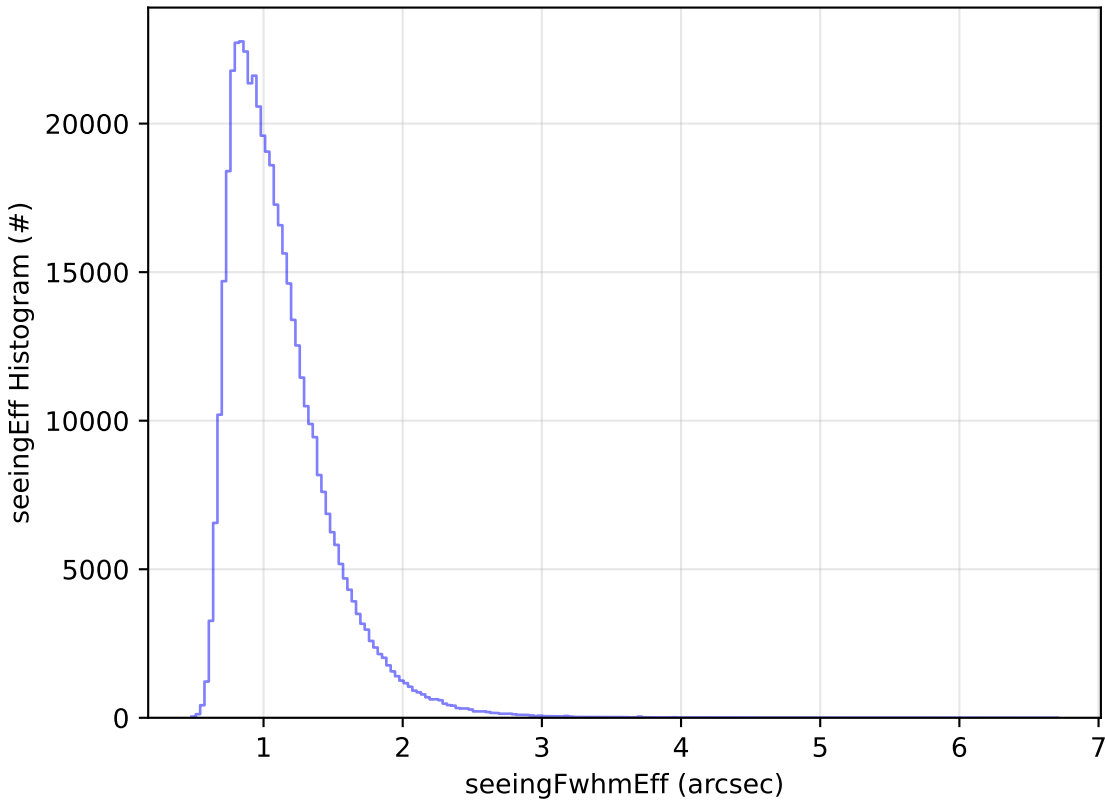
start_date_do-270v3.4_10yrs All sky r band: seeingEff Histogram
