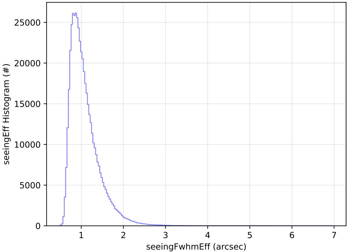
start_date_do-270v3.4_10yrs All sky i band: seeingEff Histogram
