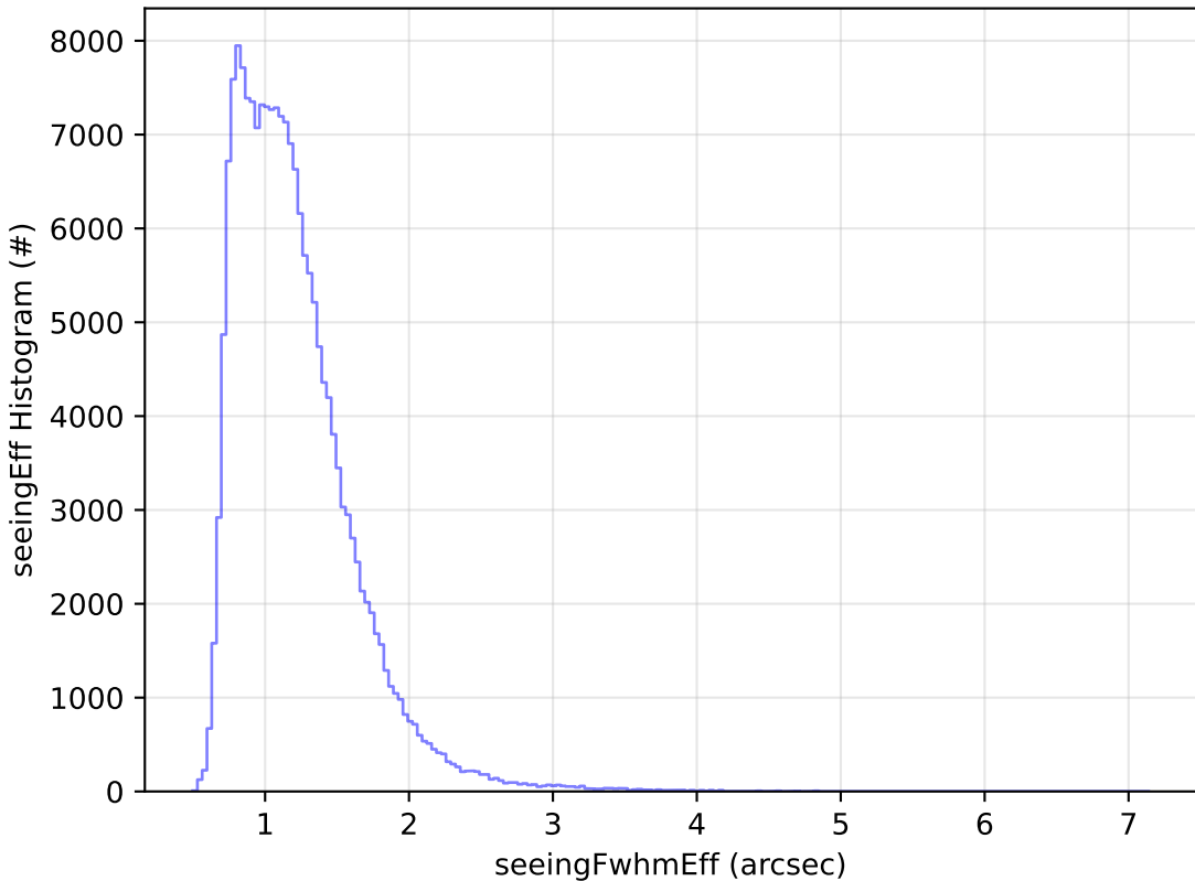
start_date_do-270v3.4_10yrs All sky g band: seeingEff Histogram
