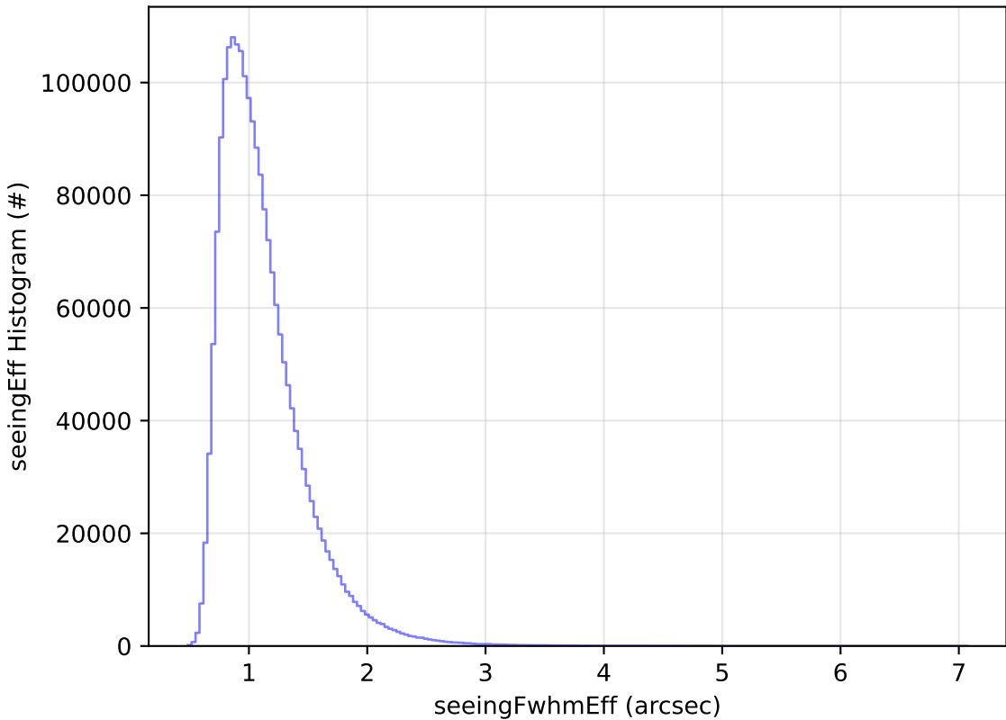
start_date_do-270v3.4_10yrs All sky all bands: seeingEff Histogram
