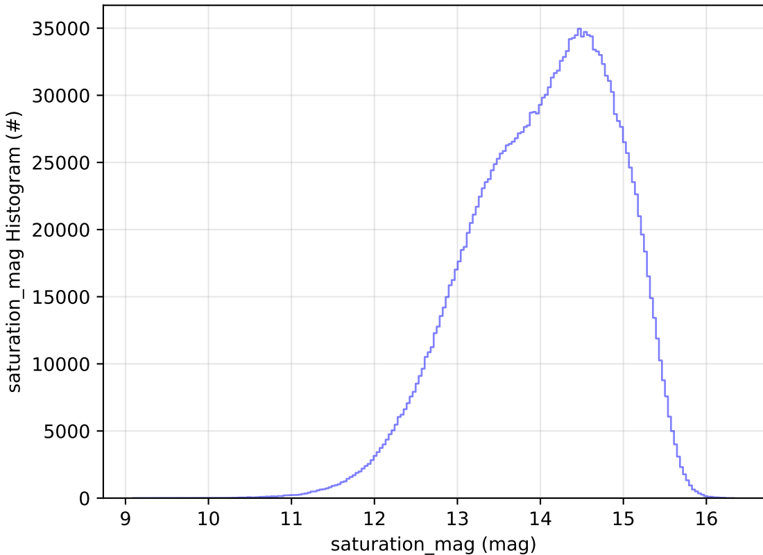
start_date_do-270v3.4_10yrs WFD all bands: saturation_mag Histogram
