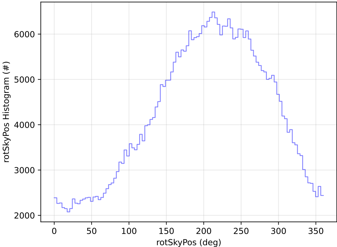
start_date_do-270v3.4_10yrs WFD z band: rotSkyPos Histogram
