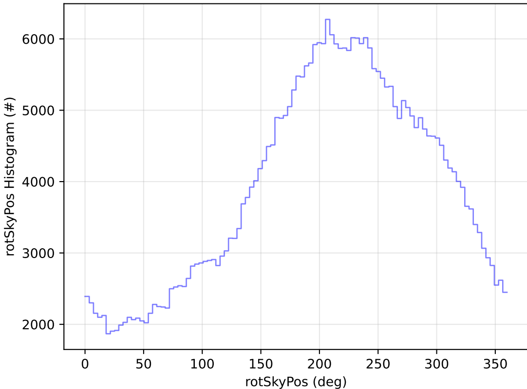
start_date_do-270v3.4_10yrs WFD y band: rotSkyPos Histogram
