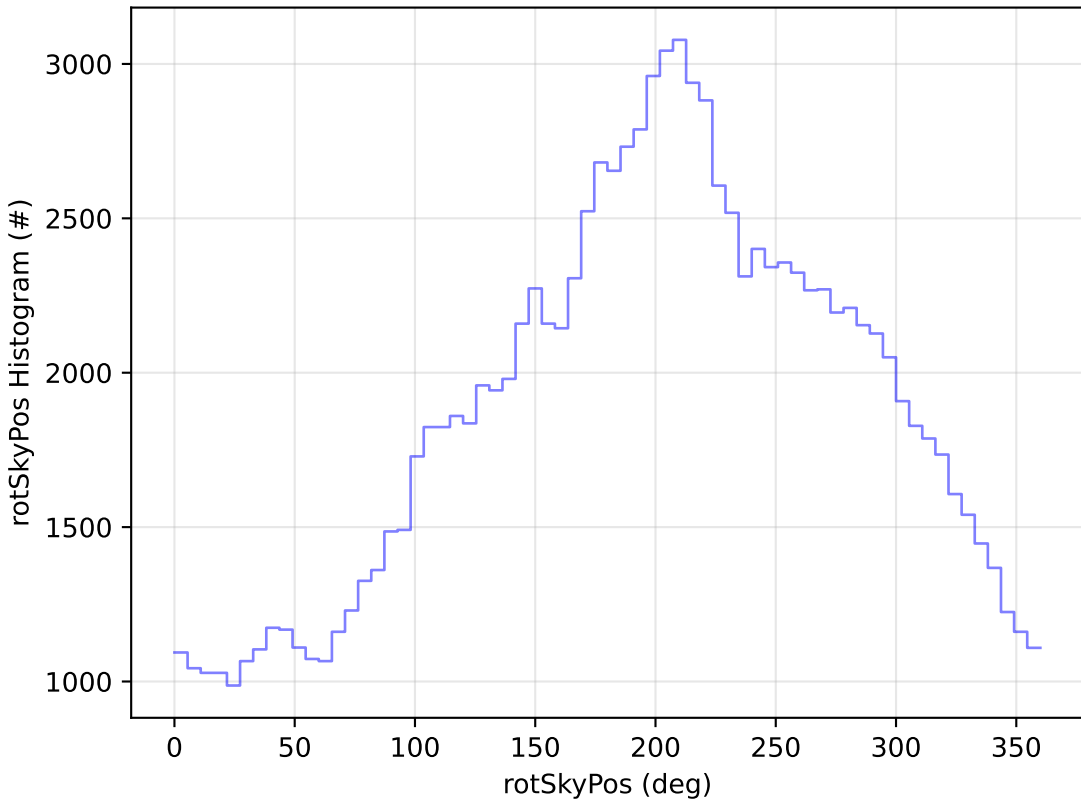
start_date_do-270v3.4_10yrs WFD u band: rotSkyPos Histogram
