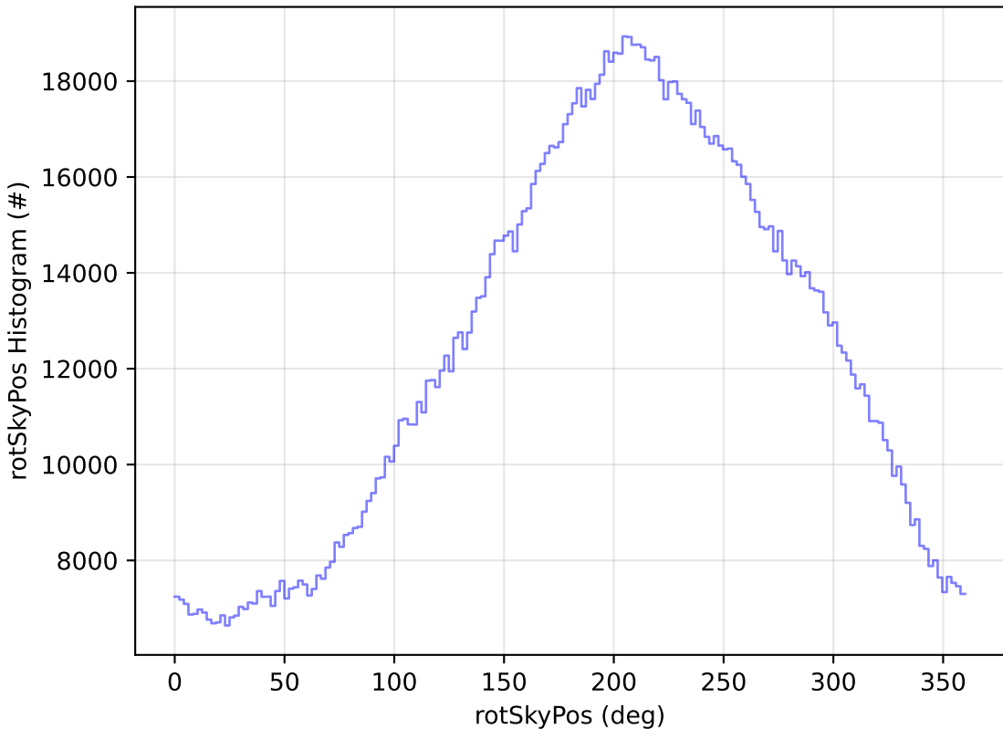
start_date_do-270v3.4_10yrs WFD all bands: rotSkyPos Histogram
