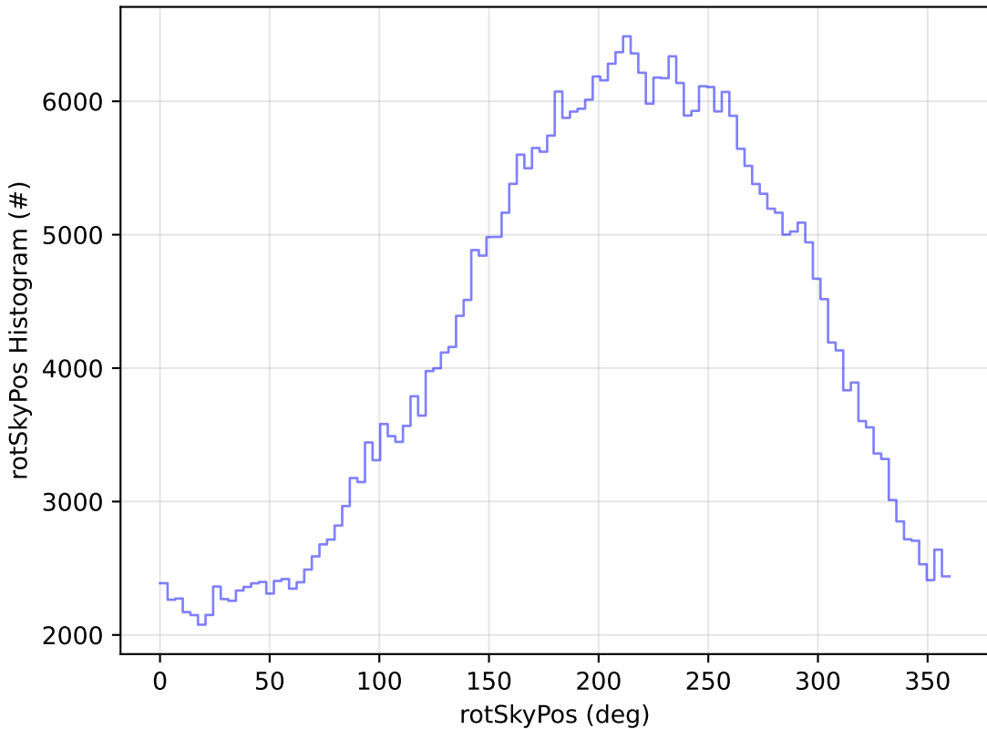
start_date_do-270v3.4_10yrs All sky z band: rotSkyPos Histogram
