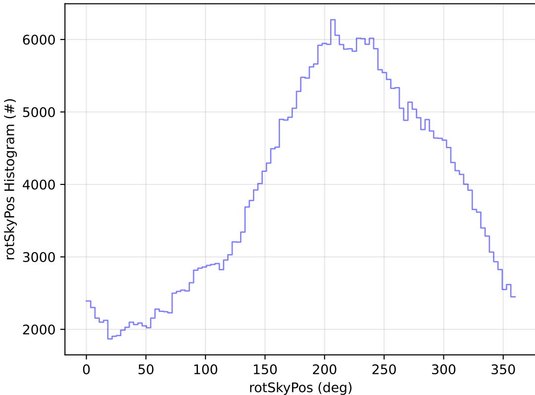
start_date_do-270v3.4_10yrs All sky y band: rotSkyPos Histogram
