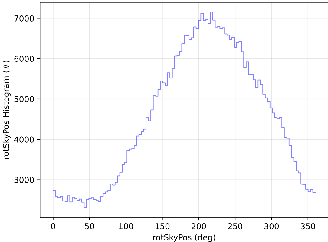
start_date_do-270v3.4_10yrs All sky i band: rotSkyPos Histogram
