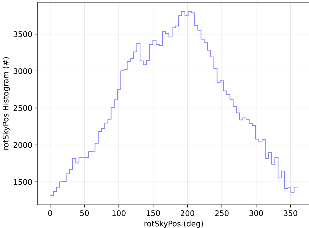
start_date_do-270v3.4_10yrs All sky g band: rotSkyPos Histogram
