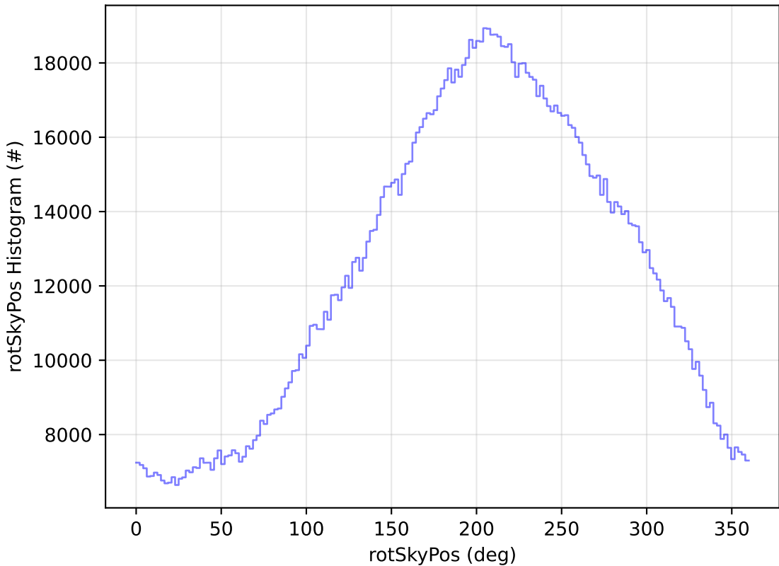
start_date_do-270v3.4_10yrs All sky all bands: rotSkyPos Histogram
