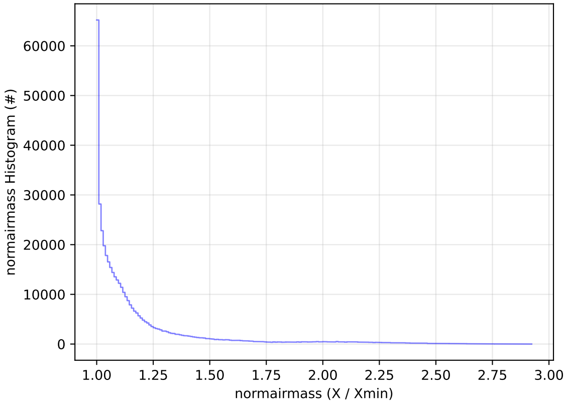
start_date_do-270v3.4_10yrs WFD z band: normairmass Histogram
