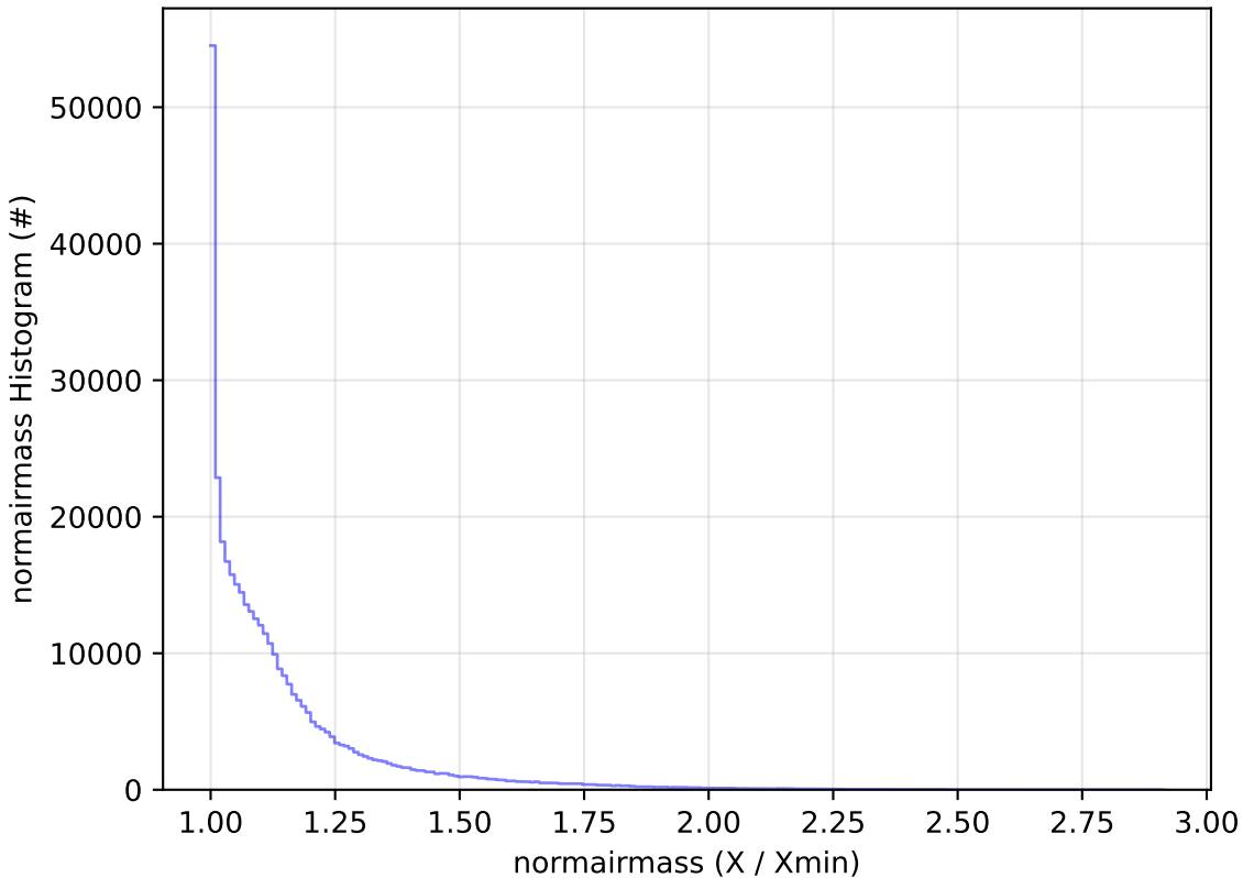
start_date_do-270v3.4_10yrs WFD y band: normairmass Histogram
