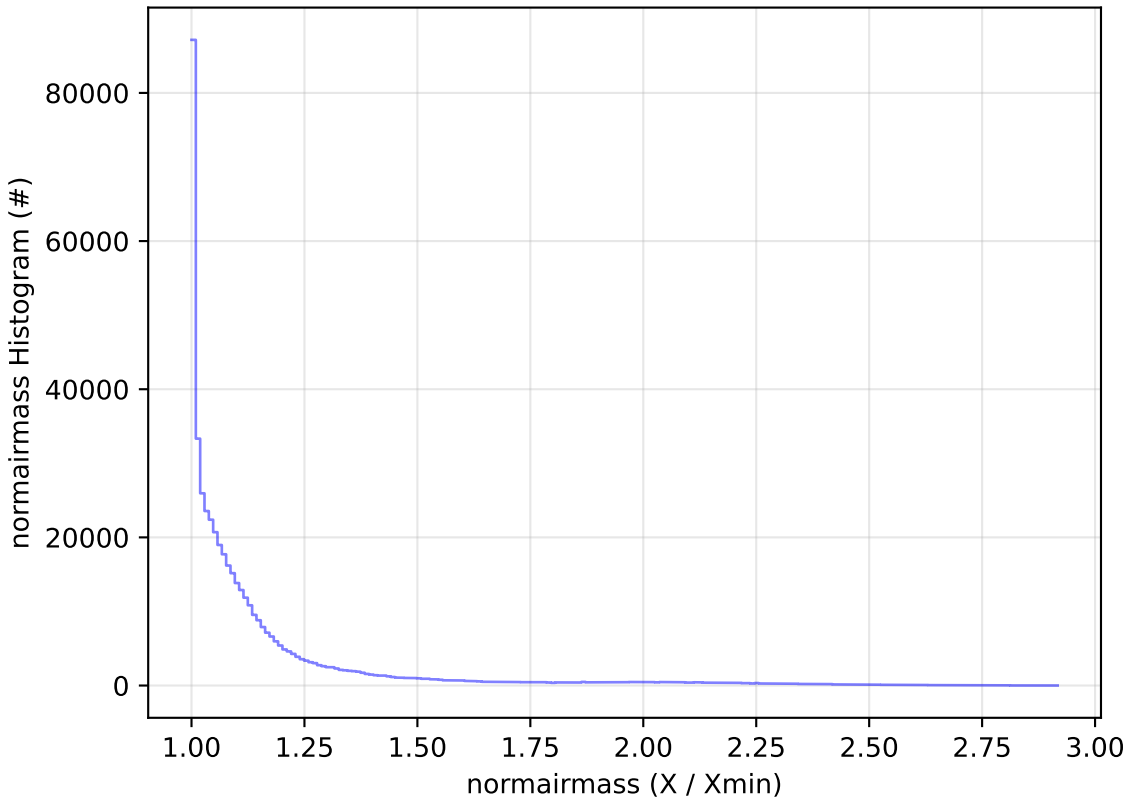
start_date_do-270v3.4_10yrs WFD i band: normairmass Histogram
