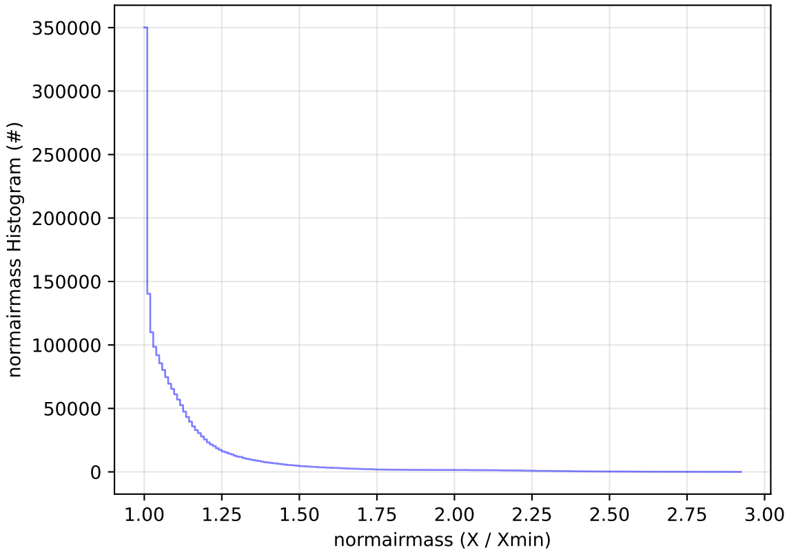
start_date_do-270v3.4_10yrs WFD all bands: normairmass Histogram
