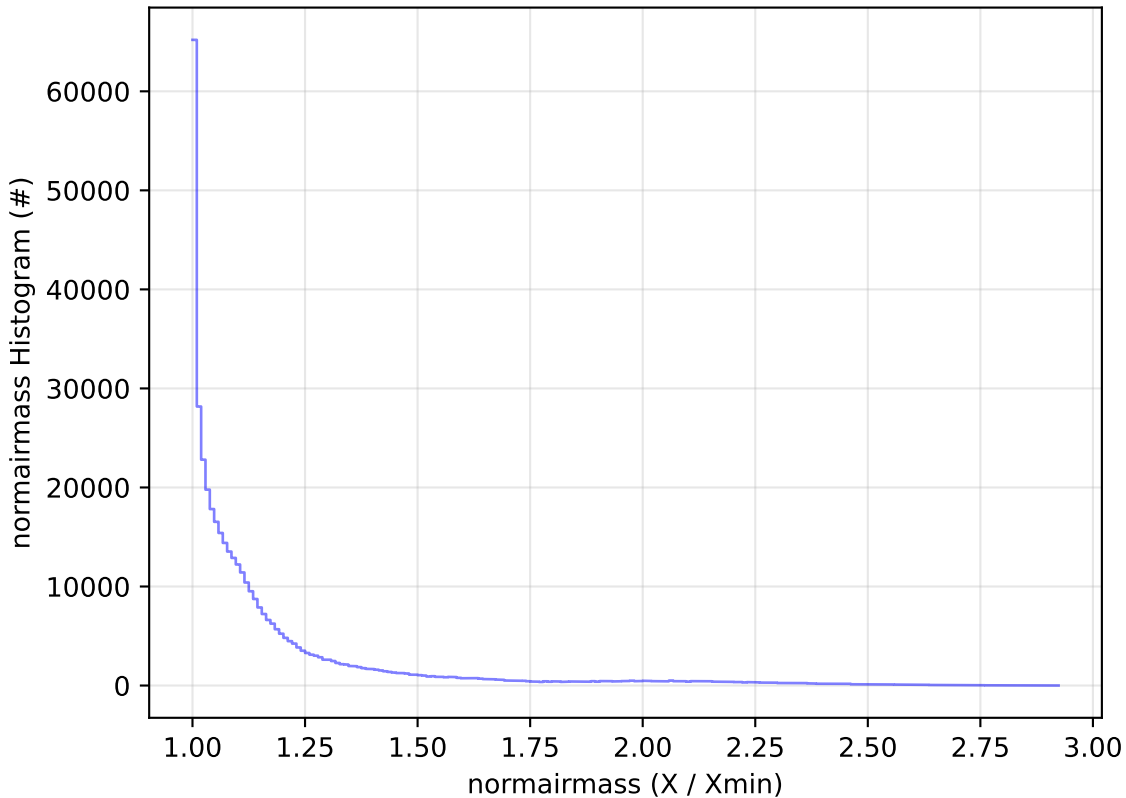
start_date_do-270v3.4_10yrs All sky z band: normairmass Histogram
