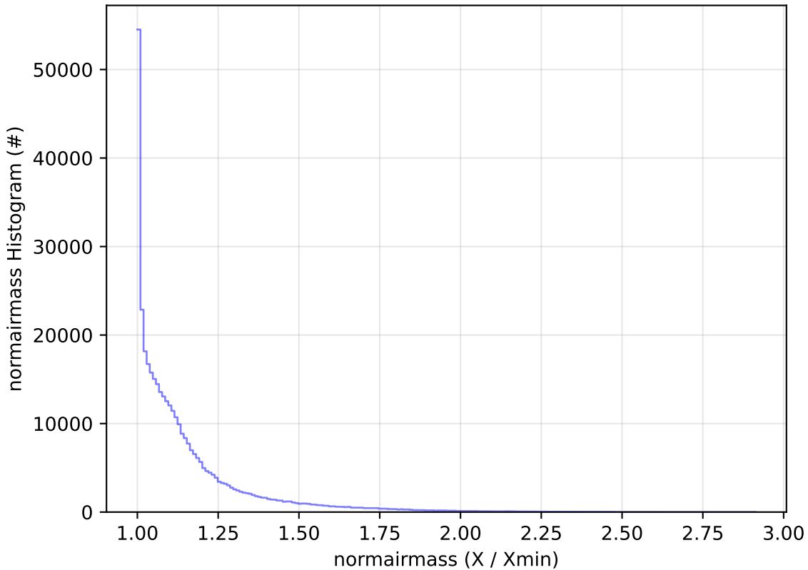
start_date_do-270v3.4_10yrs All sky y band: normairmass Histogram
