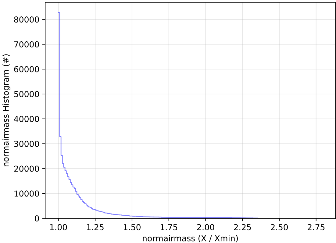
start_date_do-270v3.4_10yrs All sky r band: normairmass Histogram
