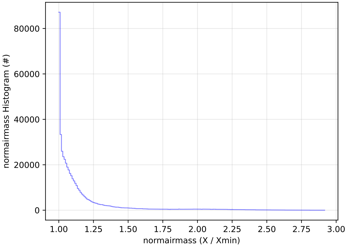
start_date_do-270v3.4_10yrs All sky i band: normairmass Histogram
