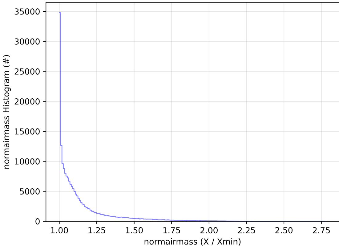
start_date_do-270v3.4_10yrs All sky g band: normairmass Histogram
