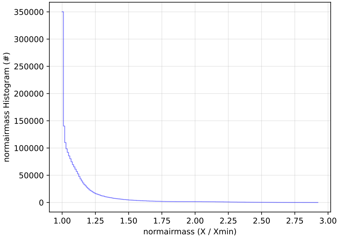
start_date_do-270v3.4_10yrs All sky all bands: normairmass Histogram
